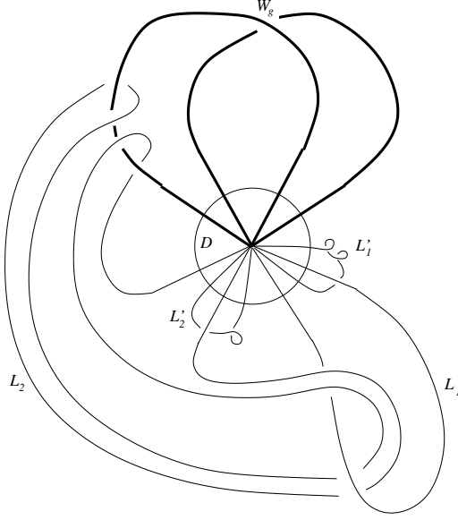
FIGURE 1. An example of a bouquet W and D \cap W
