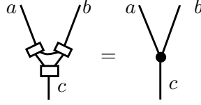
FIGURE 4. A skin element (left) is recovered from a colored trivalent graph (right) by replacing a vertex locally by the skin element in K(\mathcal{D}^2) with a + b marked points above and c points below.
