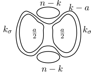
FIGURE 17. The crossingless skein \overline{J_\sigma(a)} .
