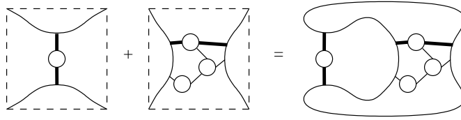
FIGURE 4. An example of unexpected losses. Upon tangle addition, the dark edges connect the same pair of vertices.
