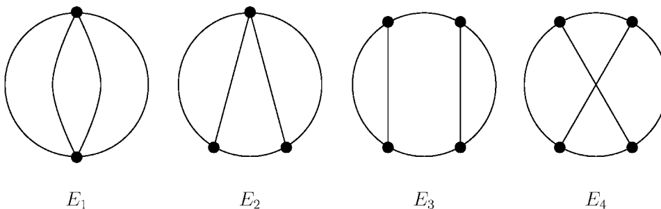
FIGURE 4. The multigraphs for l = 2 .
