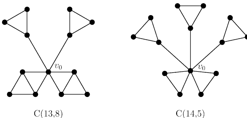
FIGURE 2. Examples of C(n, r) for n < 3r .
