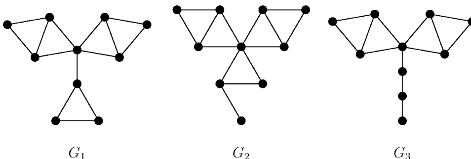
FIGURE 9. Three graphs to eliminate.
