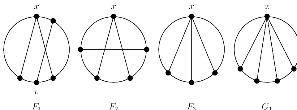
FIGURE 5. Three children and one grandchild of E_2 .
