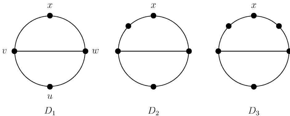
FIGURE 8. Three special subdivisions of D .
