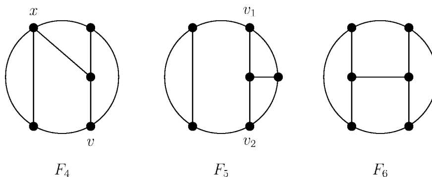
FIGURE 6. Three children of E_3 .
